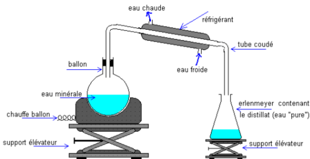
Figure 13 : L'hydrodistillation
